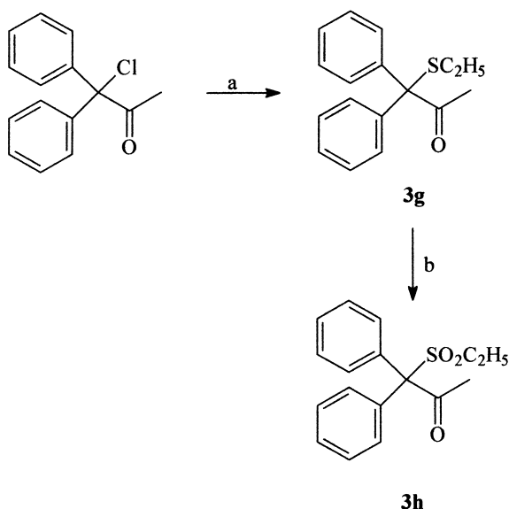
Scheme 2. (a) \text{C}_2\text{H}_5\text{SH} , \text{CaCO}_3 , 80^\circ\text{C} , (b) MCPBA, \text{CH}_2\text{Cl}_2 , rt.
