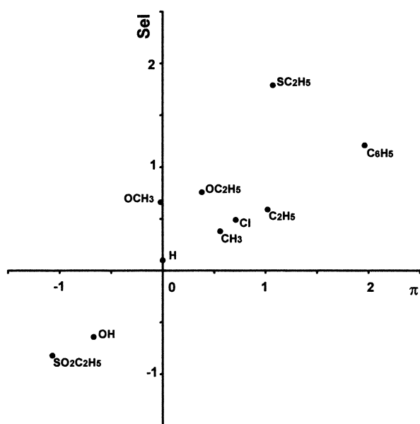
Figure 3. Plot of the M_2/M_3 selectivity (Sel) versus lipophilicity ( \pi ).
