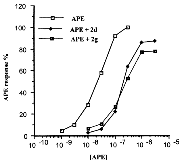
Figure 2. Experimental dose–response curves of APE on guinea-pig ileum ( M_3 ) in the absence ( \square ) and in the presence of 10\ \mu\text{M} of 2d ( \blacklozenge ) and 2g ( \blacksquare ). The decrease of the maximum effect of APE suggests a non-competitive behavior of the two antagonists.
