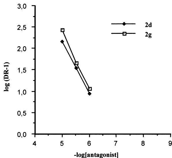
Figure 1. Schild plots obtained for the antagonists 2d and 2g on guinea-pig atria force ( M_2 ). The points are the means of five to seven experiments. S.E.M.s are not reported for clarity and are less than 10%. Ordinate: \log(\text{DR}-1) where \text{DR} = \text{EC}_{50} ratio measured from the displacement of the agonist concentration–response curves by the antagonist. Abscissa: -\log[\text{antagonist}] . Schild correlations, based on three points, do not deviate from linearity, suggesting a competitive behavior of the two antagonists.
